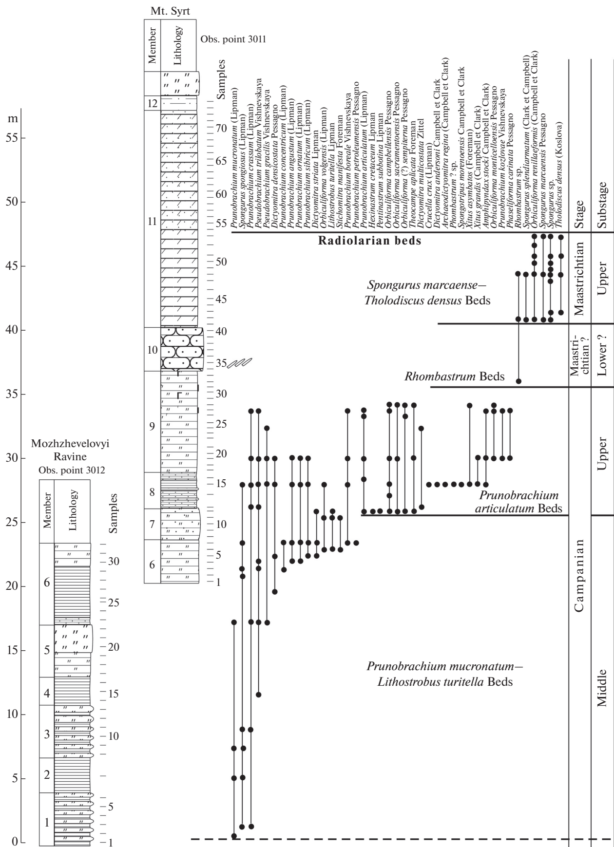
Fig. 5. Radiolarians in the Nizhnyaya Bannovka section (distribution, assemblages, and assumed age).
