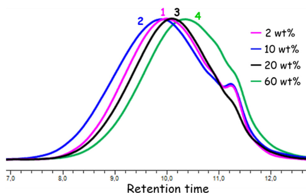
Figure 3. GPC curves obtained in Experiments 1–4.
