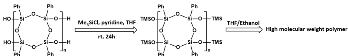
Scheme 1. Blocking of residual silanol groups in L-PPSQ and followed by reprecipitation of the resulting polymers.
