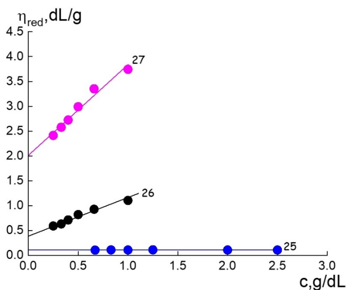
Figure 14. Reduced viscosity vs. concentration for dilute solutions of polymers 25–27 in toluene (T = 37 °C).
