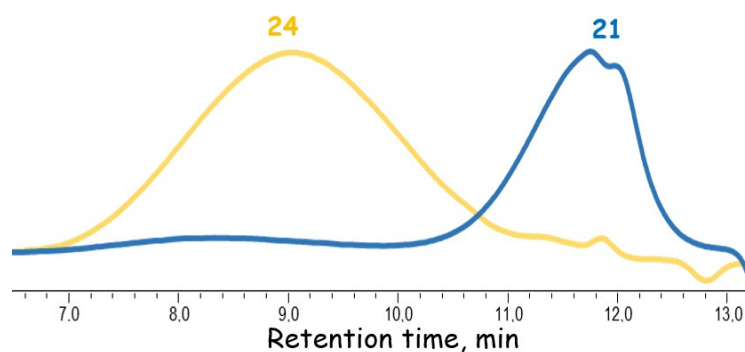
Figure 9. GPC curves obtained in Experiment 21 is the low molecular weight condensation product of cis -tetraol with addition of water; Experiment 24 is the product of condensation of sample 21.
