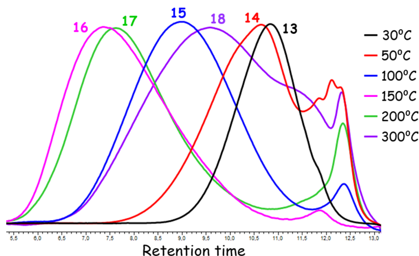
Figure 6. GPC curves obtained in Experiments 13–18.
