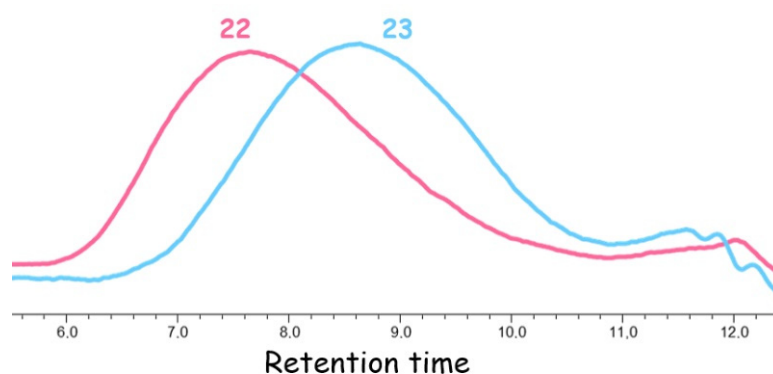
Figure 8. GPC curves obtained in Experiments 22—L-PPSQ with silanol groups blocked by trimethylchlorosilane; 23—condensation product of sample 22 with addition of water.
