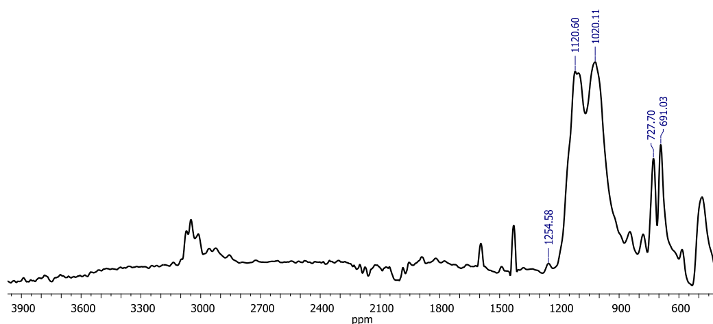
Figure 12. IR spectra of L-PPSQ 27.
