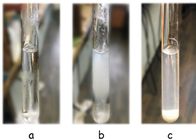
Figure 2. (a) Solubility of the monomer in ammonia, (b) 15 min after dissolution, and (c) 1 h after dissolution.
