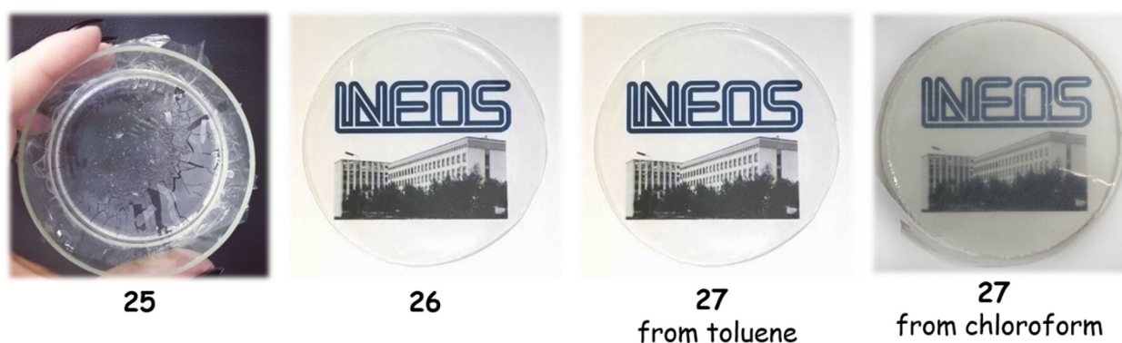
Figure 11. Polymer films 25–27.
