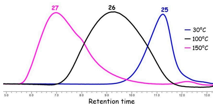
Figure 10. GPC curves obtained in Experiments 25–27.
