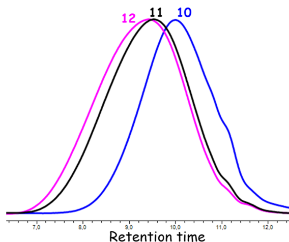
Figure 5. GPC curves obtained in experiments 10—L-PPSQ synthesis; 11—synthesis after first decompression; 12—synthesis after second decompression.
