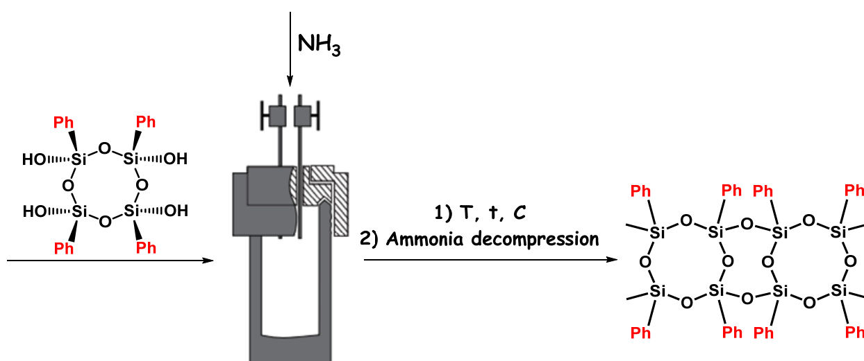
Figure 1. General scheme of L-PPSQ synthesis in ammonia medium.
