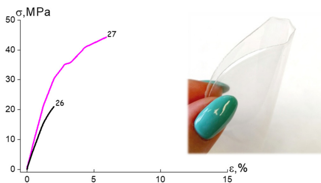
Figure 16. Stretching curves of polymers 26–27.
