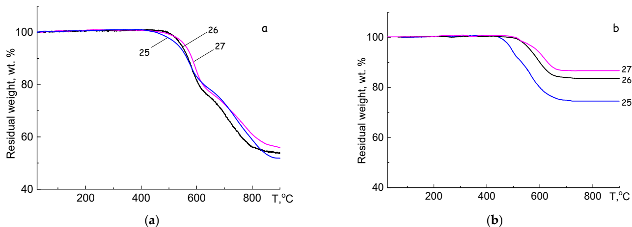
Figure 15. TGA curves of polymers 25–27 obtained at a heating rate of 10 degrees/min: (a) in air; (b) in argon.
