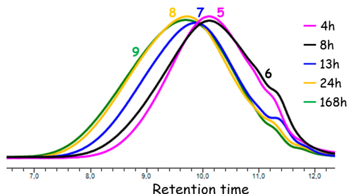
Figure 4. GPC curves obtained in Experiments 5–9.
