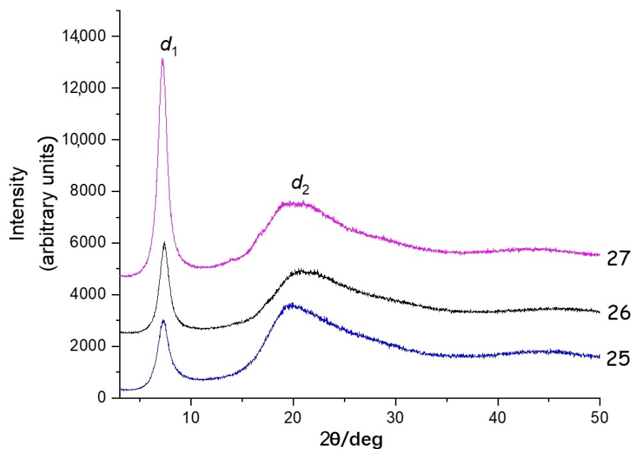
Figure 13. Diffraction data for polymers 25–27.
