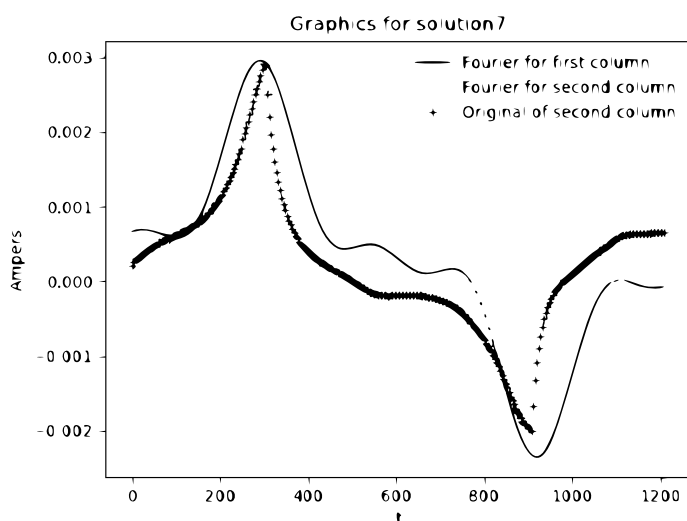
Рис. 1. The thick line depicts the graph of the function y_k obtained pointwise from the matrix AG, the thin line is the graph of the function y_k(t) , the dotted line is the graph of the function \tilde{y}_k(t)
