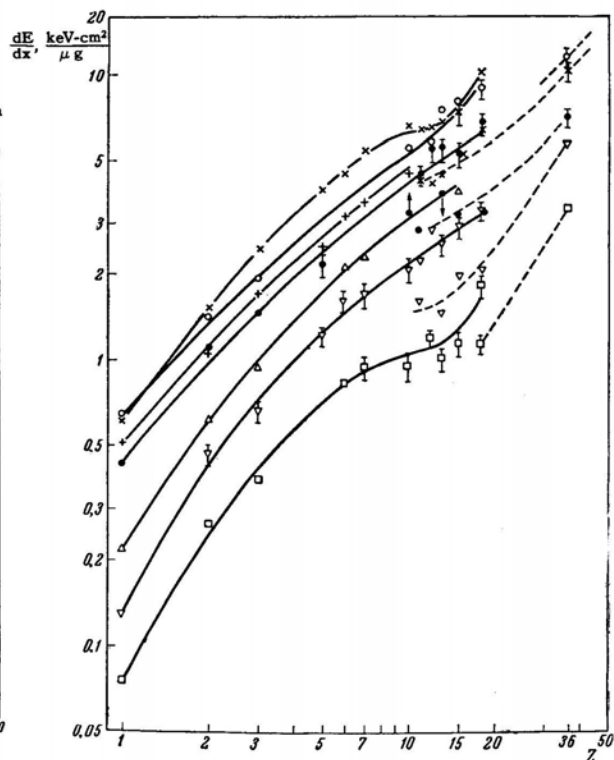
FIG. 5. Dependence of dE/dx on Z . \times in air, + in argon, \circ in celluloid, \bullet in Al, \triangle in Ni, \nabla in Ag, \square in Au. Continuous lines — v = 3.7 \times 10^8 cm/sec; dashed lines — v = 2.35 \times 10^8 cm/sec. The vertical bars represent maximum errors.
