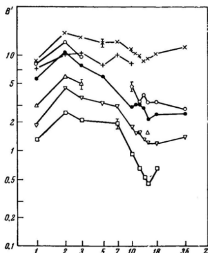
FIG. 7. Dependence of B' = (dE/dx)/i^2 on Z : \times in air, o in celluloid, + in argon, \bullet in Al, \Delta in Ni, \nabla in Ag, \square in Au. v = 3.7 \times 10^8 cm/sec.
