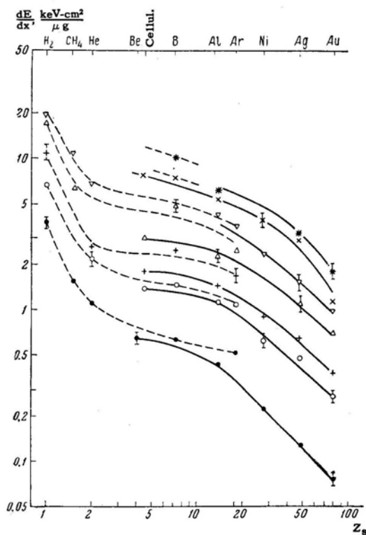
FIG. 6. Dependence of dE/dx on Z_s for ions: \bullet - protons, \circ - He, + - Li, \Delta - B, \nabla - N, \times - P, * - Ar; v = 3.7 \times 10^8 cm/sec. Continuous lines - in solids; dashed lines - in gases.
