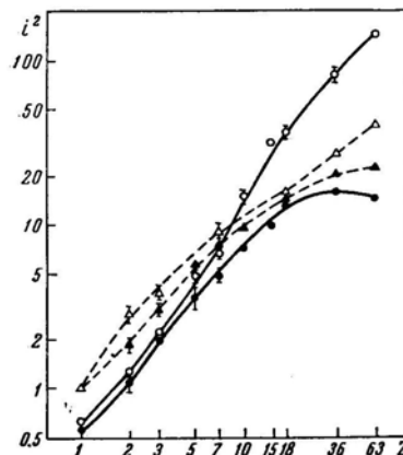
FIG. 8. Dependence of i^2 (continuous lines) and of i^{*2} (dashed lines) on Z at v = 3.16 \times 10^8 cm/sec. \circ and \bullet denote i^2 in solids and gases, respectively; \Delta and \blacktriangle denote i^{*2} in solids and gases, respectively. The data for fission fragments ( Z \sim 63 ) were taken from [11] and [25] .
