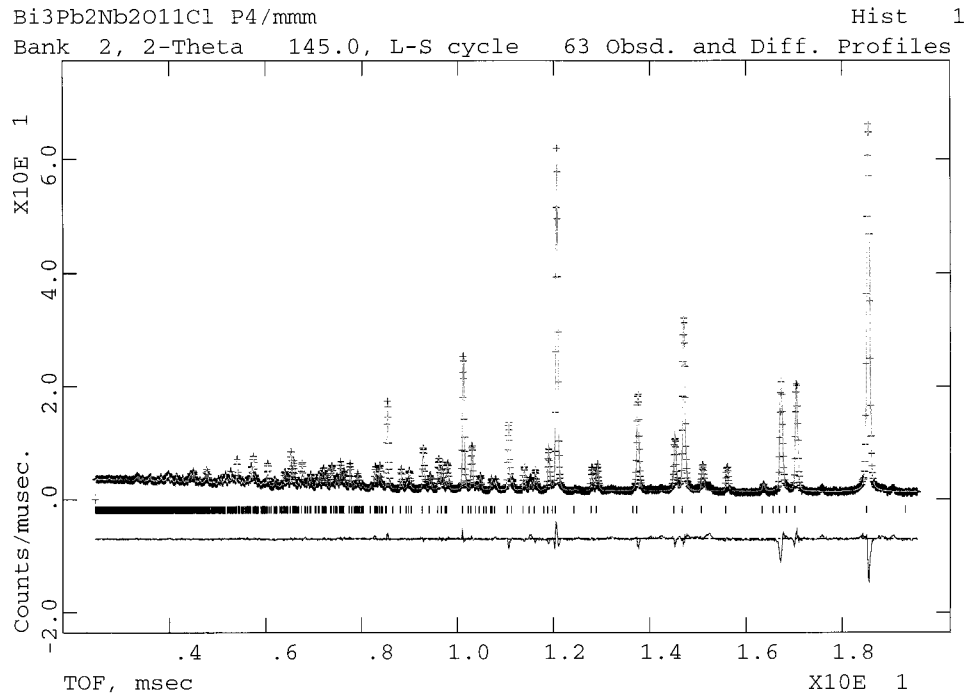
Figure 5. Final Rietveld plot for the powder neutron diffraction refinement of Bi 3 Pb 2 Nb 2 O 11 Cl.
