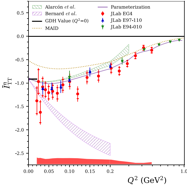
FIG. 23. EG4 results on the neutron \bar{T}_{TT}^n(Q^2) , compared with results from JLab E94-010 ( ^3\text{He} ) [92] (green triangles) and E97-110 ( ^3\text{He} ) [71] (blue triangles). Across all Q^2 bins, the size of the systematic uncertainty varies from 0.0275 to 0.141, while the relative size of the systematic to statistical uncertainty varies within (49–123)%. The GDH value is shown as the short horizontal line at \bar{T}_{TT}^n(0) = -0.915 . Note that earlier CLAS data [102] and the phenomenological model predictions [55,57] are not available for this integral. See Fig. 16 caption for more details.
