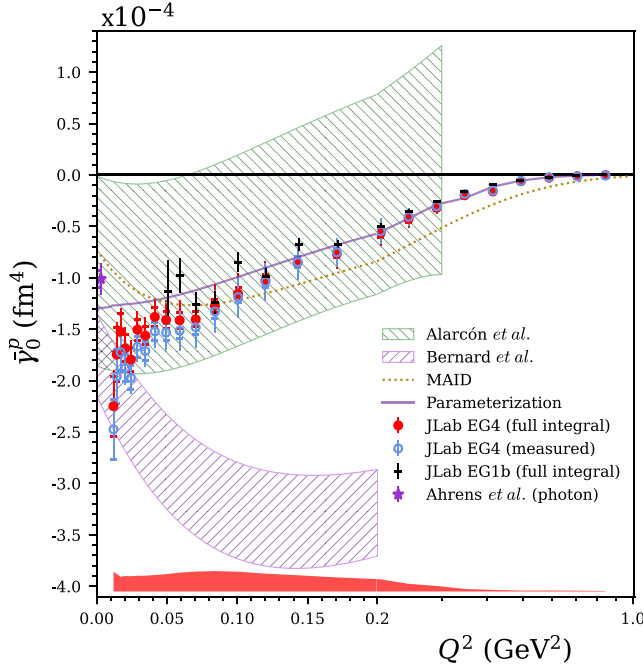
FIG. 18. EG4 results on the proton \bar{\gamma}_0^p(Q^2) . Across all Q^2 bins, the size of the systematic uncertainty (red colored band) varies from 0.0045 to 0.198 ( \times 10^{-4} fm ^4 ), while the relative size of the systematic to statistical uncertainty varies within (66–364)%. The photoproduction data point [153] is slightly displaced from Q^2 = 0 (purple star). Note that phenomenological model predictions [55,57] are not available for this integral. See Fig. 16 caption for more details.
