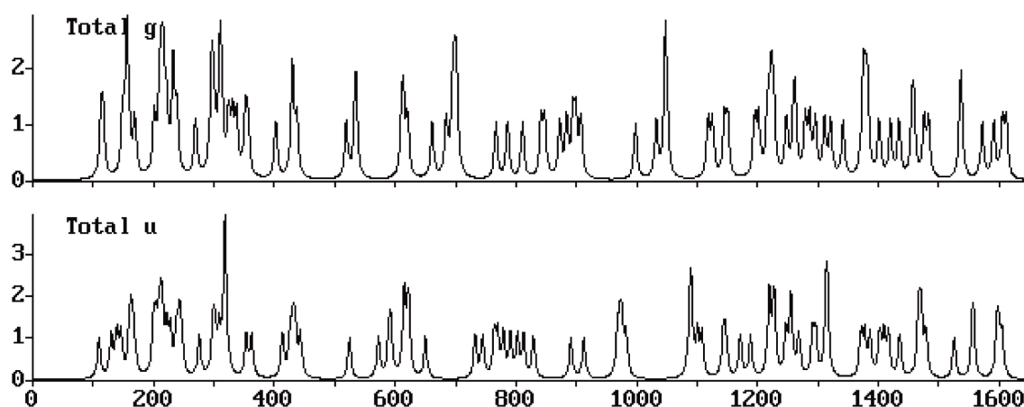
Figure 4: Vibrational state density for C_{240} molecule in the infrared absorption region between 100 and 1650 \text{cm}^{-1} .
